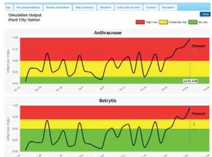
Figure 4. Model outputs in graphic formats with two days forecast.
